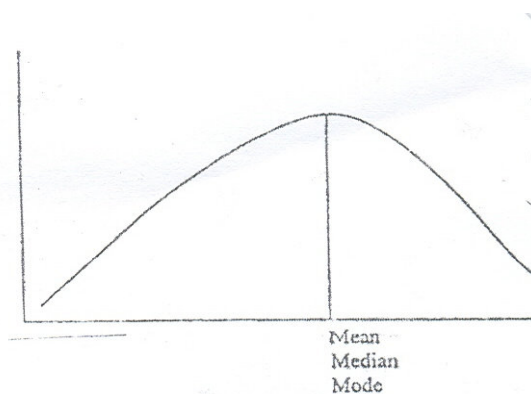
Figure 6: A Normal Distribution
