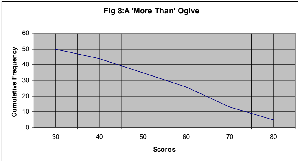
Fig. 8: A “More than” Ogive
