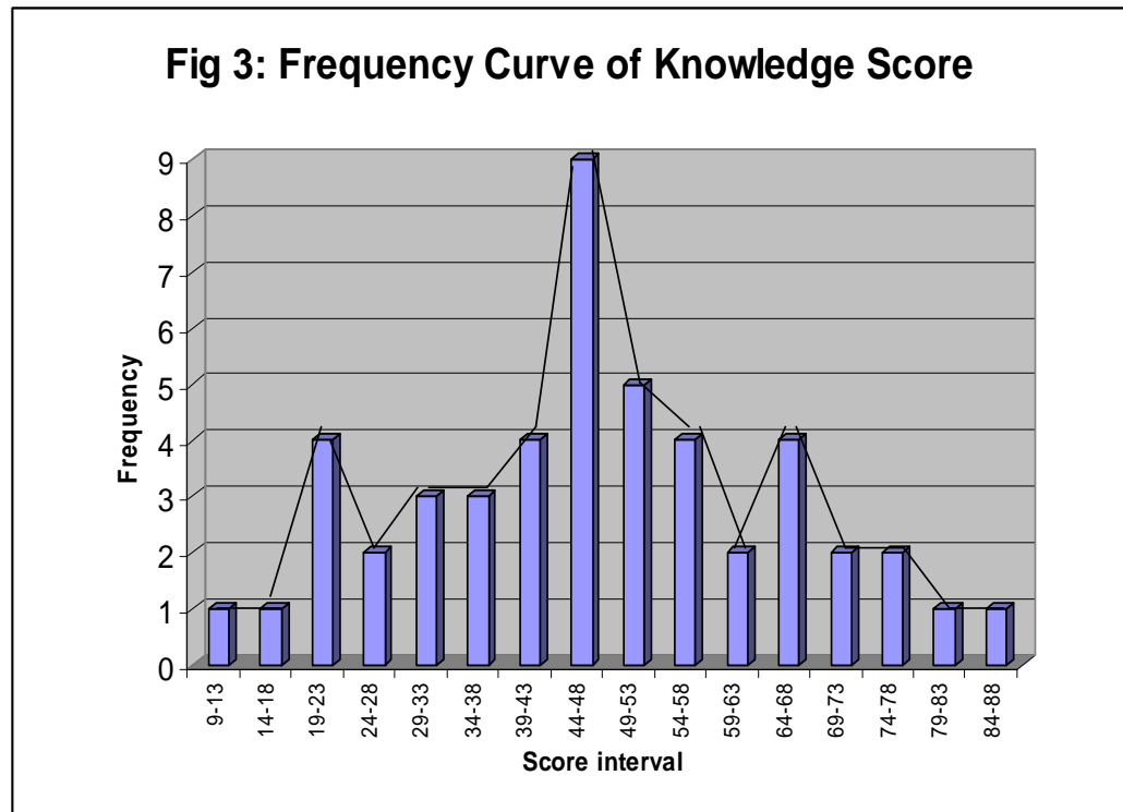
Fig. 3: Frequency Curve of knowledge Score
