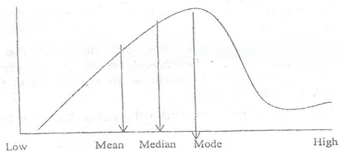
Figure 5: A Negatively Skewed Distribution
