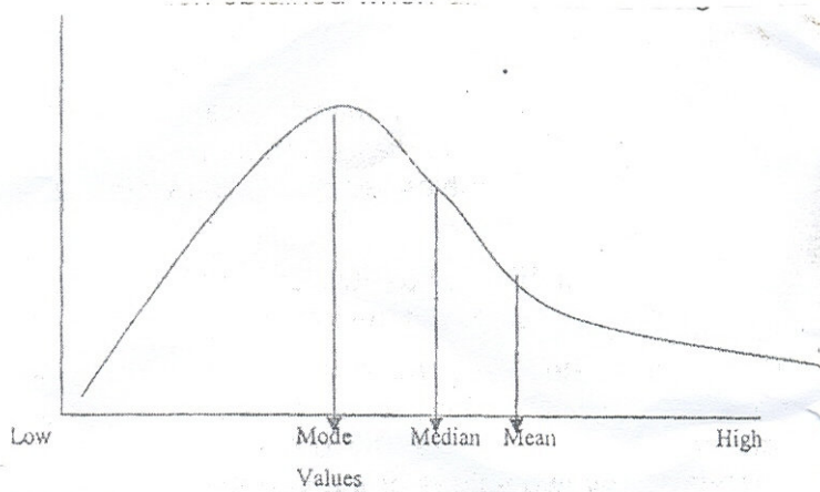
Figure 4: A Positively Skewed Distribution
