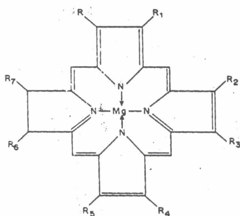
Fig 3.3: Skeleton of chlorophyll II molecule
