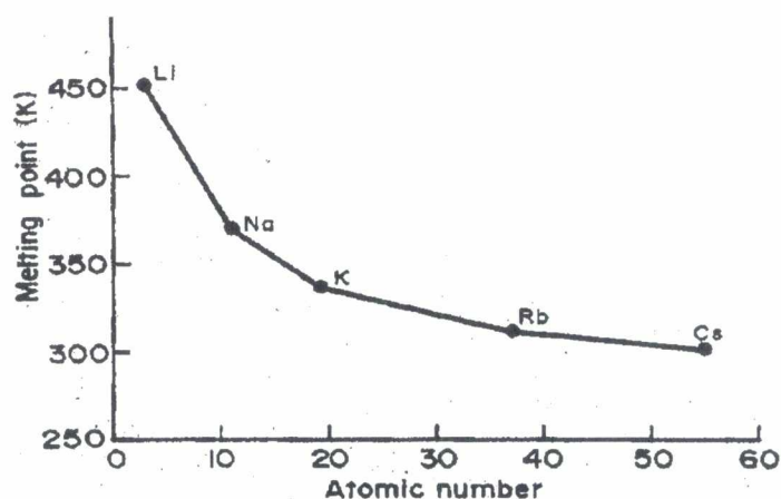
Fig 3.3: Trend in the melting point of Group 1 elements
