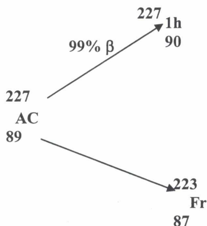
Fig. 31: Production of francium as a result of \alpha decay.
