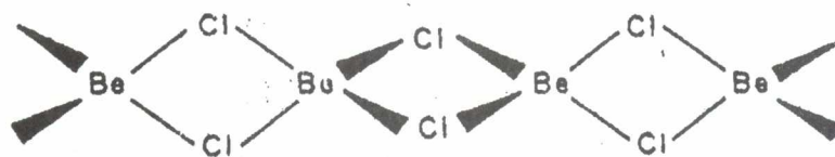
Fig 3.3: Beryllium chloride (a) monomer (m) dimer and (c) polymer
