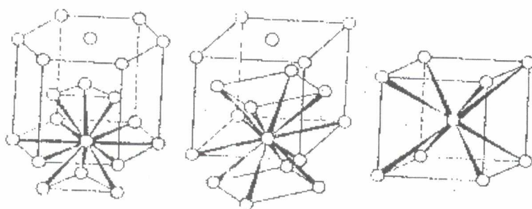
Fig. 3.2 Types of metal lattices: (a) hexagonal; (b) cubic close packed (c) body-centred cubic
