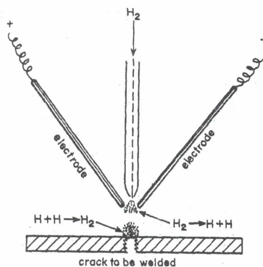
Fig. 3.1: Atomic hydrogen welding torch
