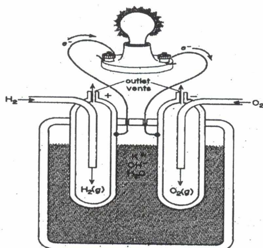
Fig 3.2: A hydrogen-oxygen fuel cell with KOH electrolyte and porous carbon electrodes
