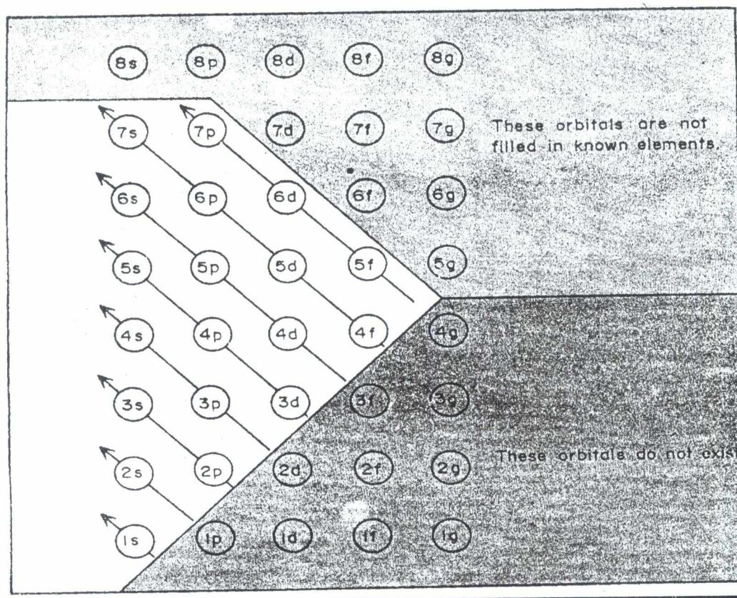
Fig 3.1: Order of filling of atomic orbitals in polyelectronic atoms
