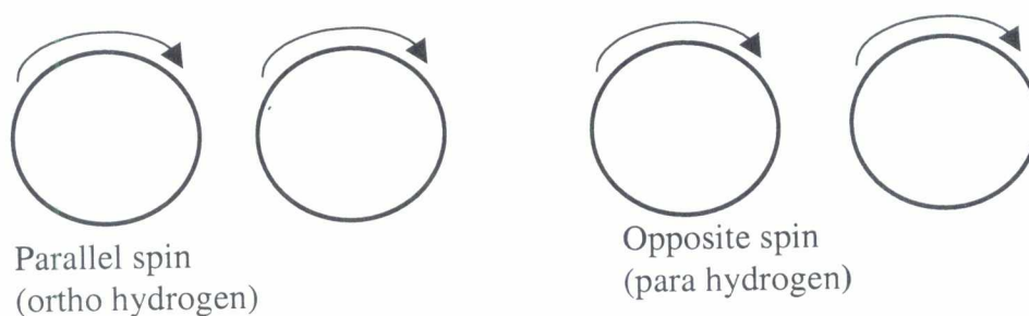
Fig. 3.2. Ortho and Para forms of hydrogen
