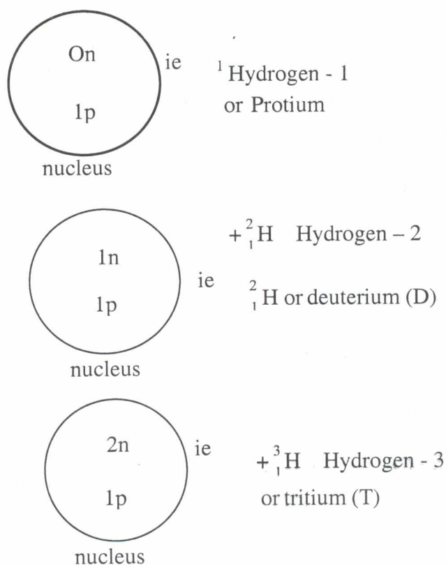
Fig 3.1 Isotopes of hydrogen
