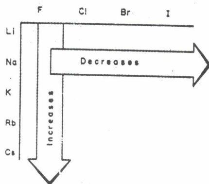
Figure 3.5: Trend in ionic character of alkali halides metals
