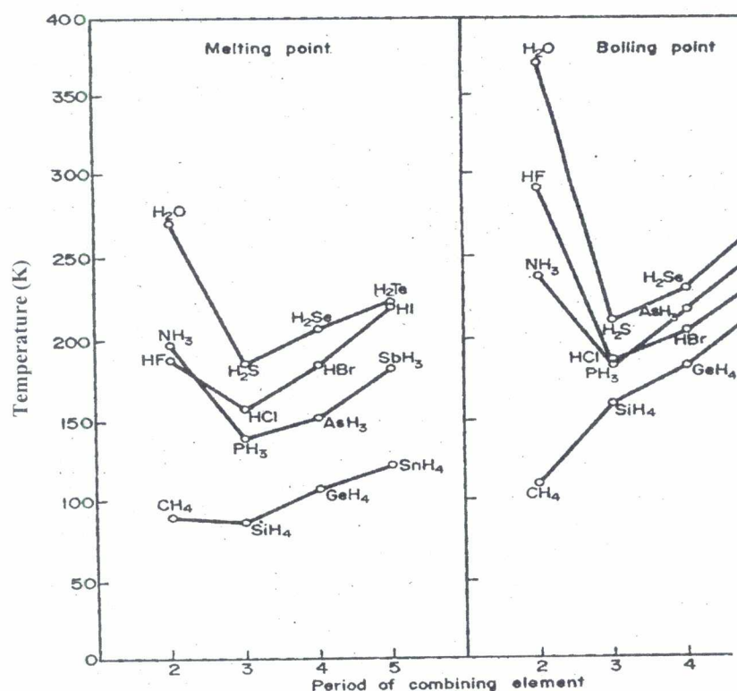
Fig. 3.1: (a) Melting point curves and (b) Boiling point curves of the molecular hydride
