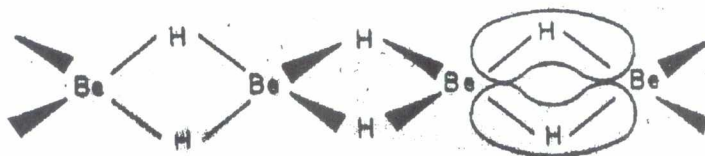
Fig 3.4: Beryllium hydride polymer
