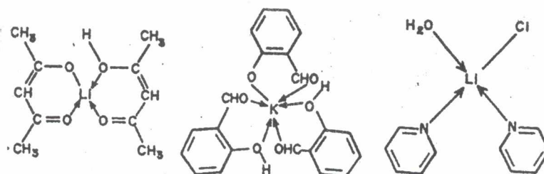
Fig 3.1: Source complex of alkali metal ions
