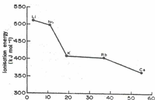
Fig 3.4: Trend in first ionization energies of alkali metals
