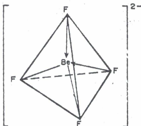
Figure 3.2 Tetrafluoroberyllate complex ion (\text{BeF}_4)^{2-}
