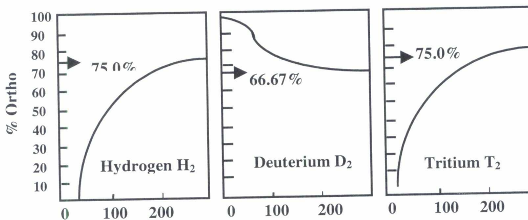
Fig. 3.3: Ortho-Para equilibria for H_2 , D_2 and T_2 ,
