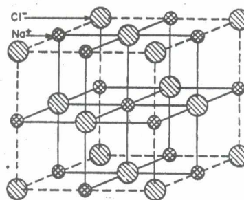
Fig 3.2: Rock salt (NaCl) structure
