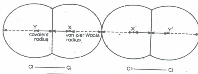
Fig 3.1: Covalent and van der Waals radii of solid chlorine
