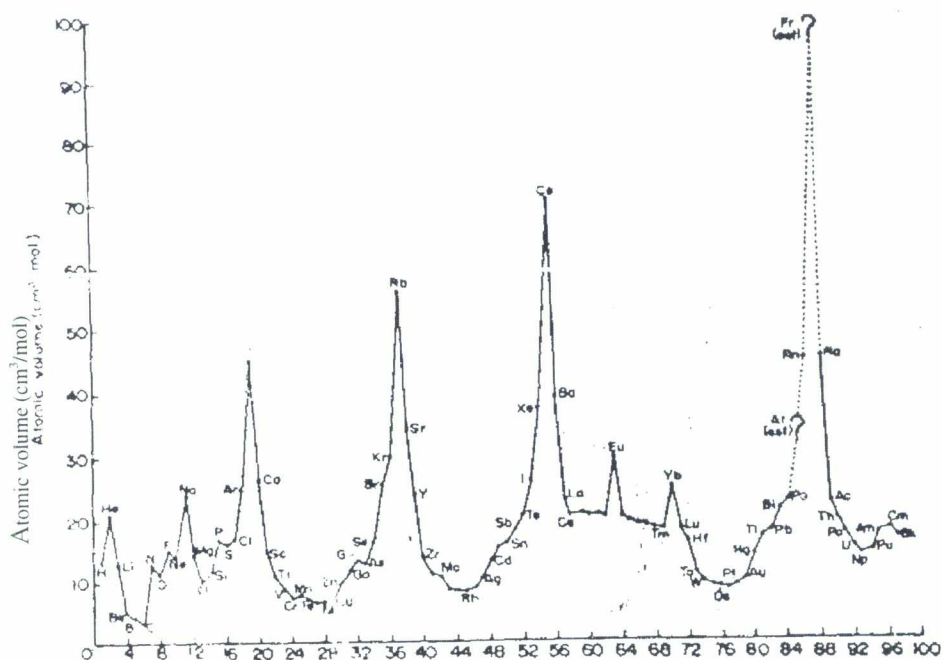
Figure 3.1 Periodic dependence of atomic volume on atomic number
