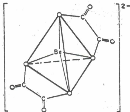
Fig 3.2: Beryllium Oxalate Complex, ion, [\text{Be}(\text{C}_2\text{O}_4)_2]^{2-}
