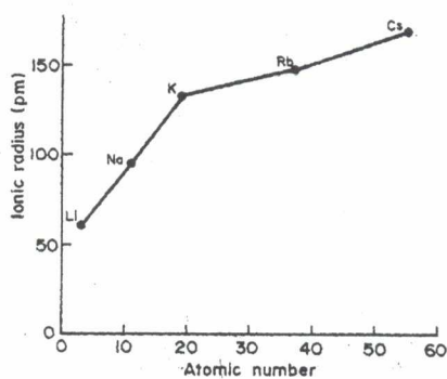
Fig. 3.2: Trend in ionic radii of Group 1 elements
