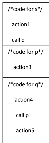
Fig. 6: Three-Address Code to Illustrate Stack Allocation
