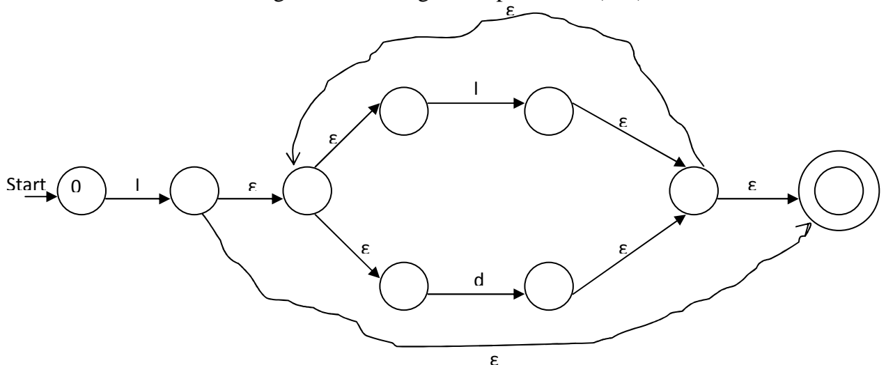
Fig. 6: NFA Recognising Identifier
