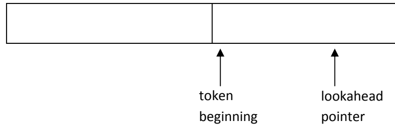
Fig. 1: Input Buffer
