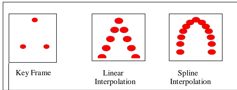
Figure .... Interpolations
