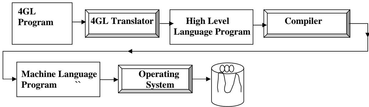
Fig. 4: Program Translation Process
