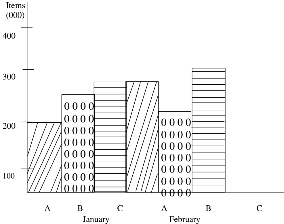
Figure 7.3 Bar Chart
