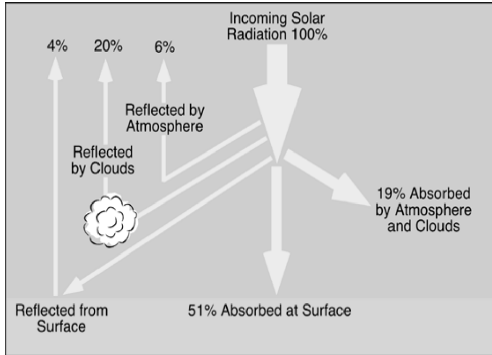
Fig. 3: Global Modification of Incoming Solar Radiation by Atmospheric and Surface Processes
