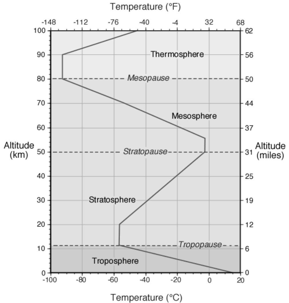
Fig. 2: Vertical Change in Average Global Atmospheric Temperature
