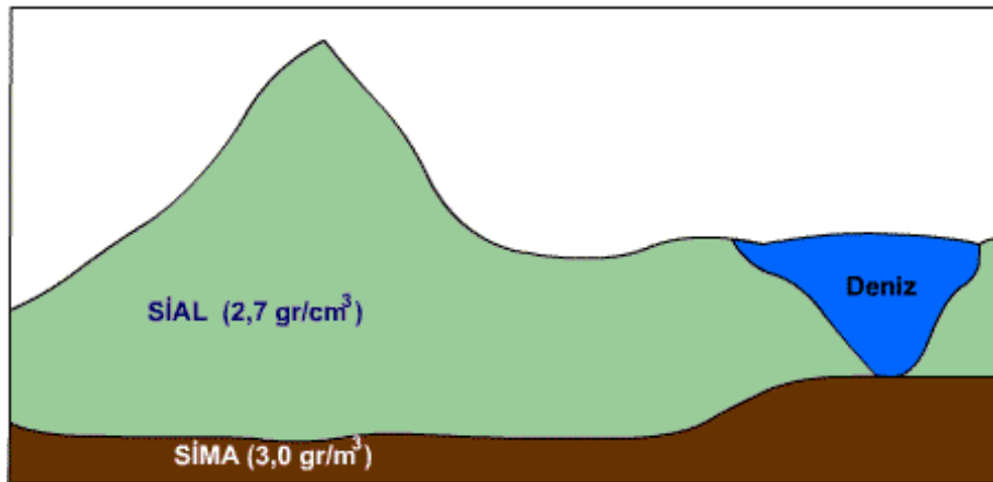
Fig. 17: SiAl resting on SiMa
