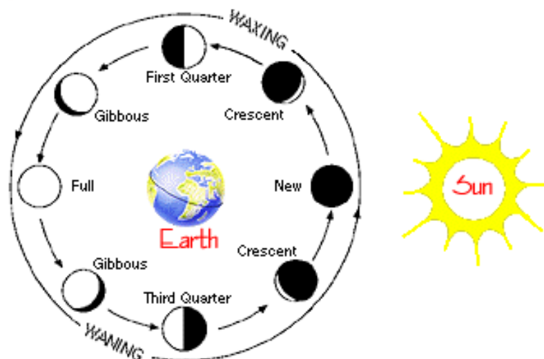
Fig. 19: Earth's Moon
