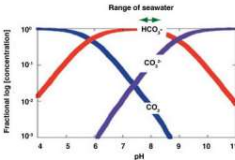
Fig. 10: Relative Proportions of Inorganic Forms of CO 2 Dissolved in Seawater
