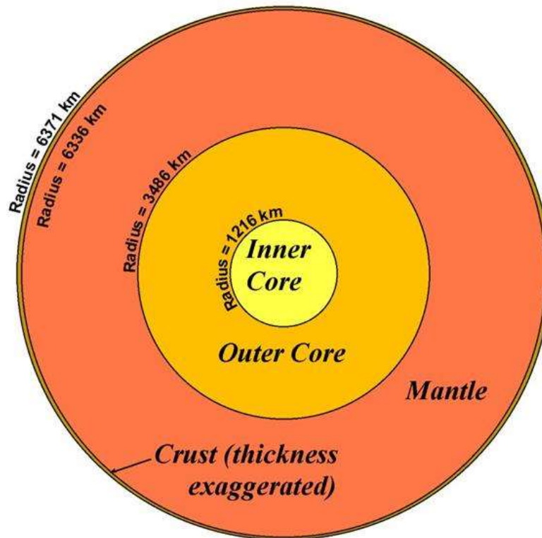
Fig. 16b: Internal and Outer Zones the Earth
