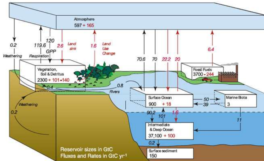
Fig. 9: Global Carbon Cycle
