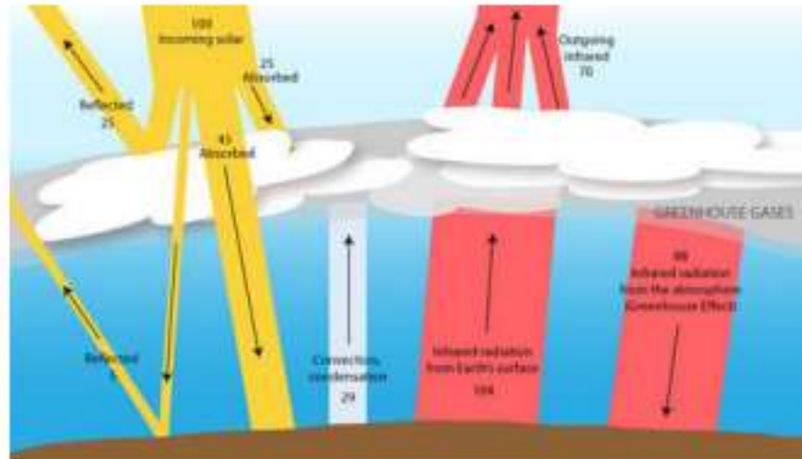
Fig. 3: Earth – Atmosphere Energy Balance
