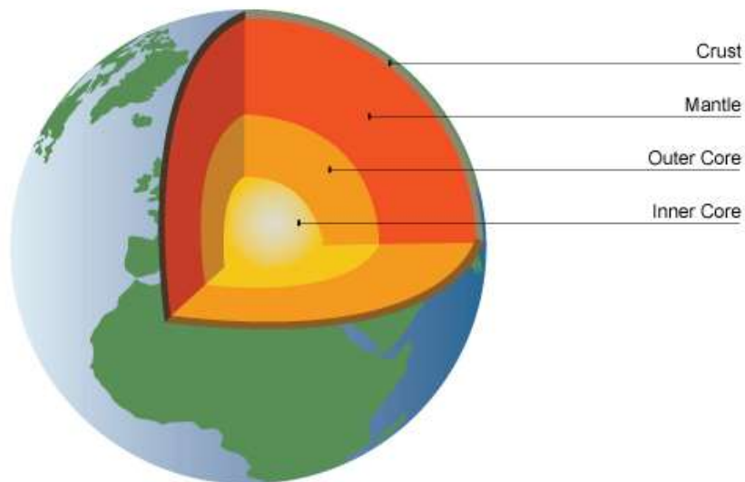
Fig. 16a: Internal Structure of the Earth
