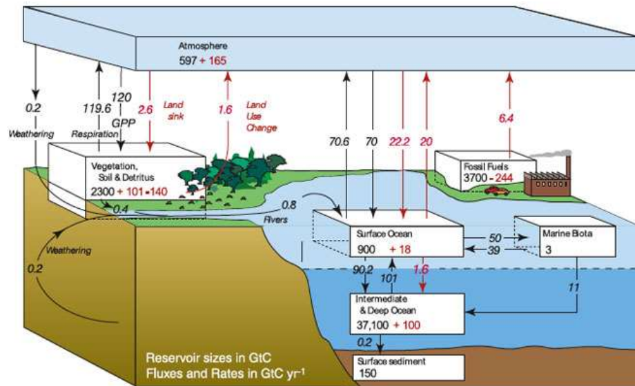
Fig 8: Global Carbon Cycle
