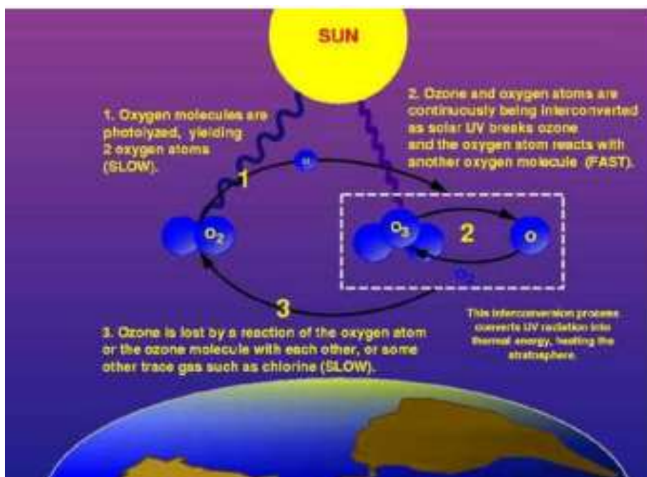
Fig. 11: Importance of Atmosphere
