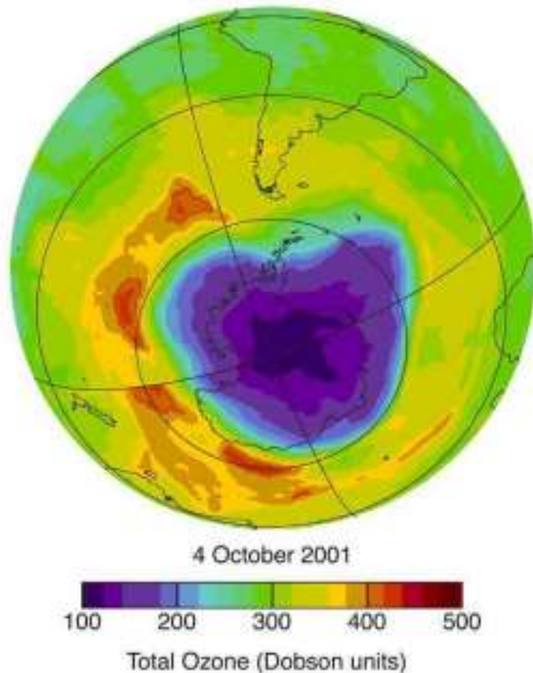
Fig. 12: Importance of Atmosphere
