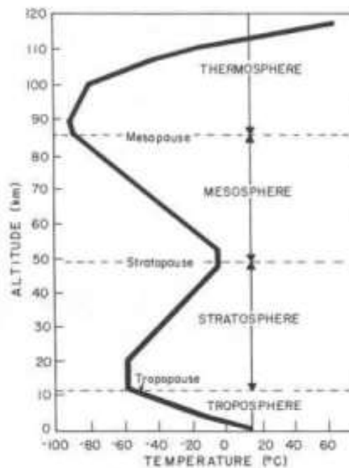
Figure 1.1: Vertical Temperature Variation of the Atmosphere and its Layers
