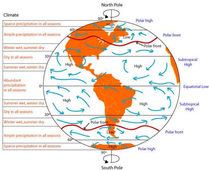
Fig. 6: Global Circulation and Climate
