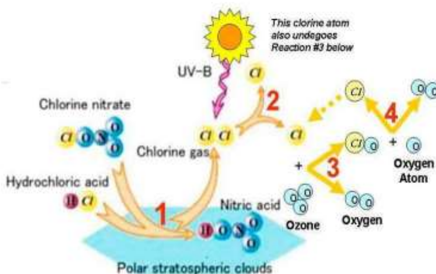
Fig. 13: Importance of Atmosphere
